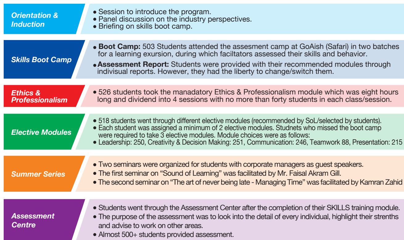
Figure 2. Program Flow
